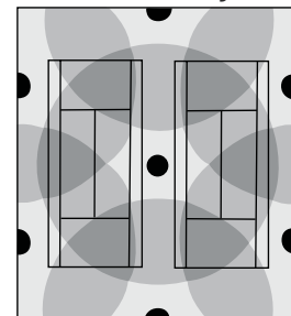
Battery of Two Courts 7- Or 8-Head Layout
