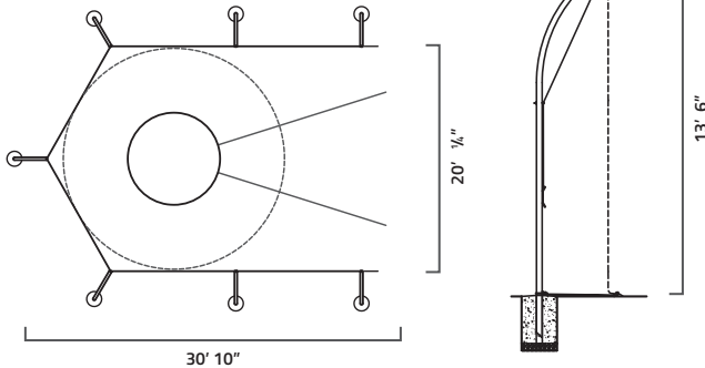
7 POLE DESIGN
