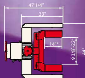
Adjustable forks
