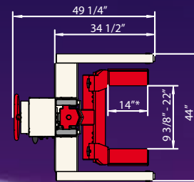
Adjustable forks
