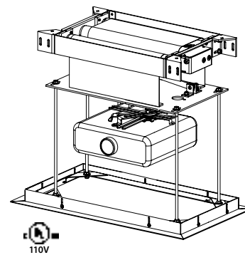
AeroLift 35 shown with optional small closure panel
