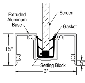
SYSTEM 350 dimensions
