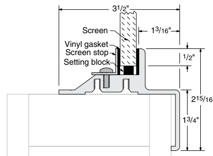
SYSTEM 400 dimensions
