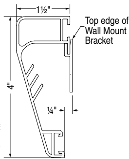
Frame Extrusion Side Detail
