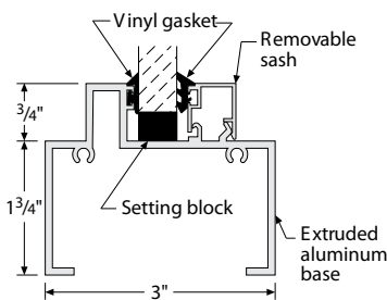
SYSTEM 200 dimensions
