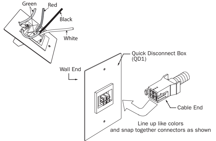
Figure 2 With optional quick disconnect wall outlet.
