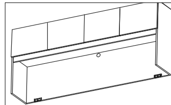
Overhead Cabinet Back Panel Grommet Back Center Pass Thru
